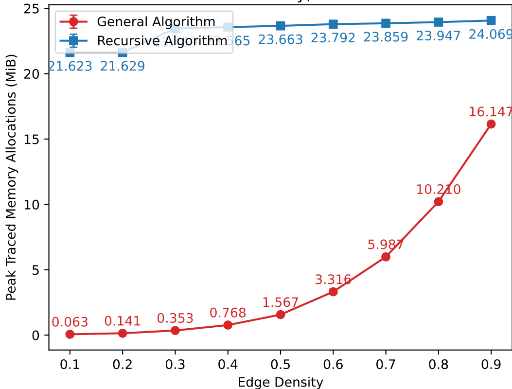
Peak Traced Allocations with Basis Tracking (10 isolated realizations per density)
